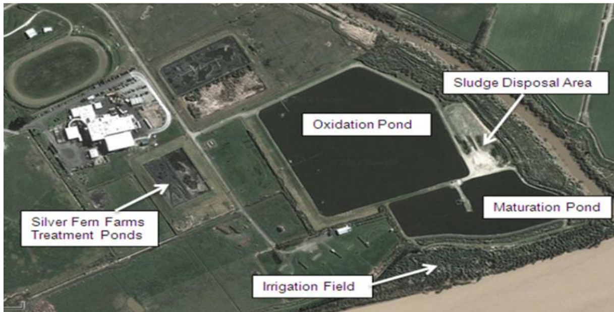
Figure 8-2: Dargaville WWTP layout (KDC Asset Management Plan 2015)
