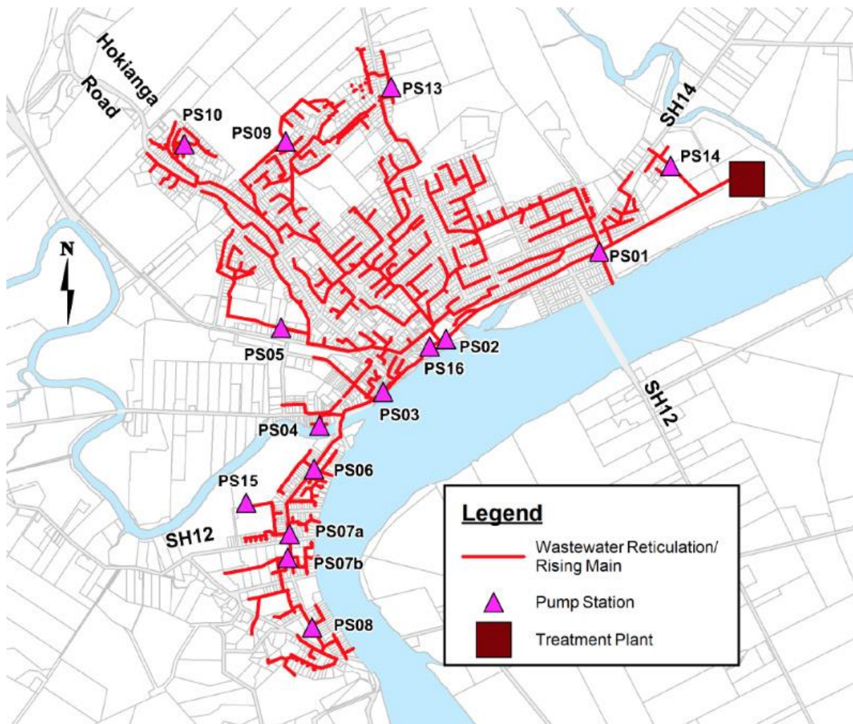
Figure 8-1: Existing Wastewater Network (KDC Asset Management Plan 2015)
